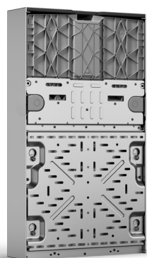
Wall-mount brackets
